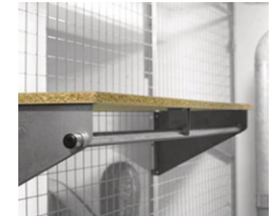
FLEXIBLE CHIPBOARD SHELF With brackets.
